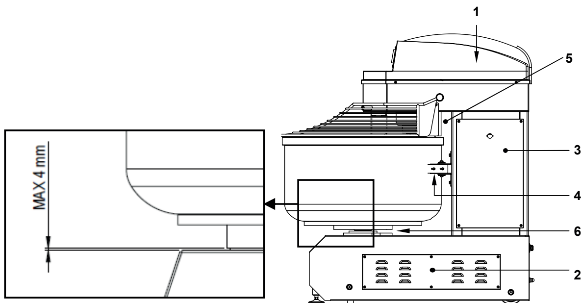
Figure 23 - Guards fixed with screws or similar devices
