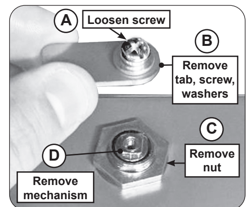
Fig. 4-5 Locking / unlocking
