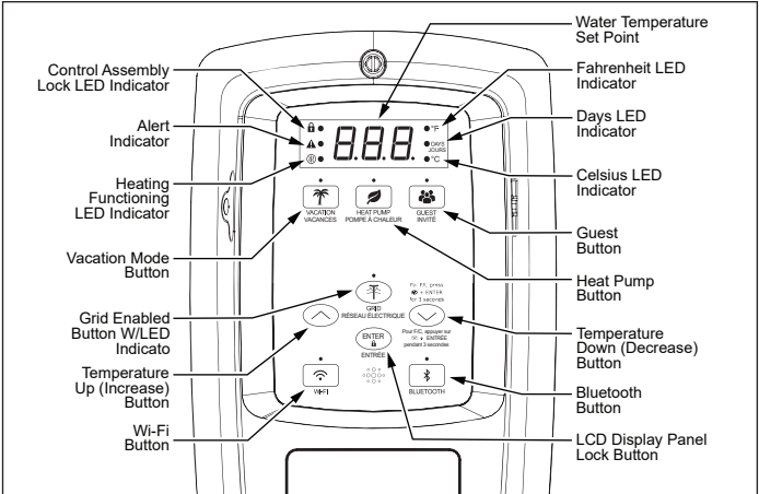
Figure 26 - Control Assembly
