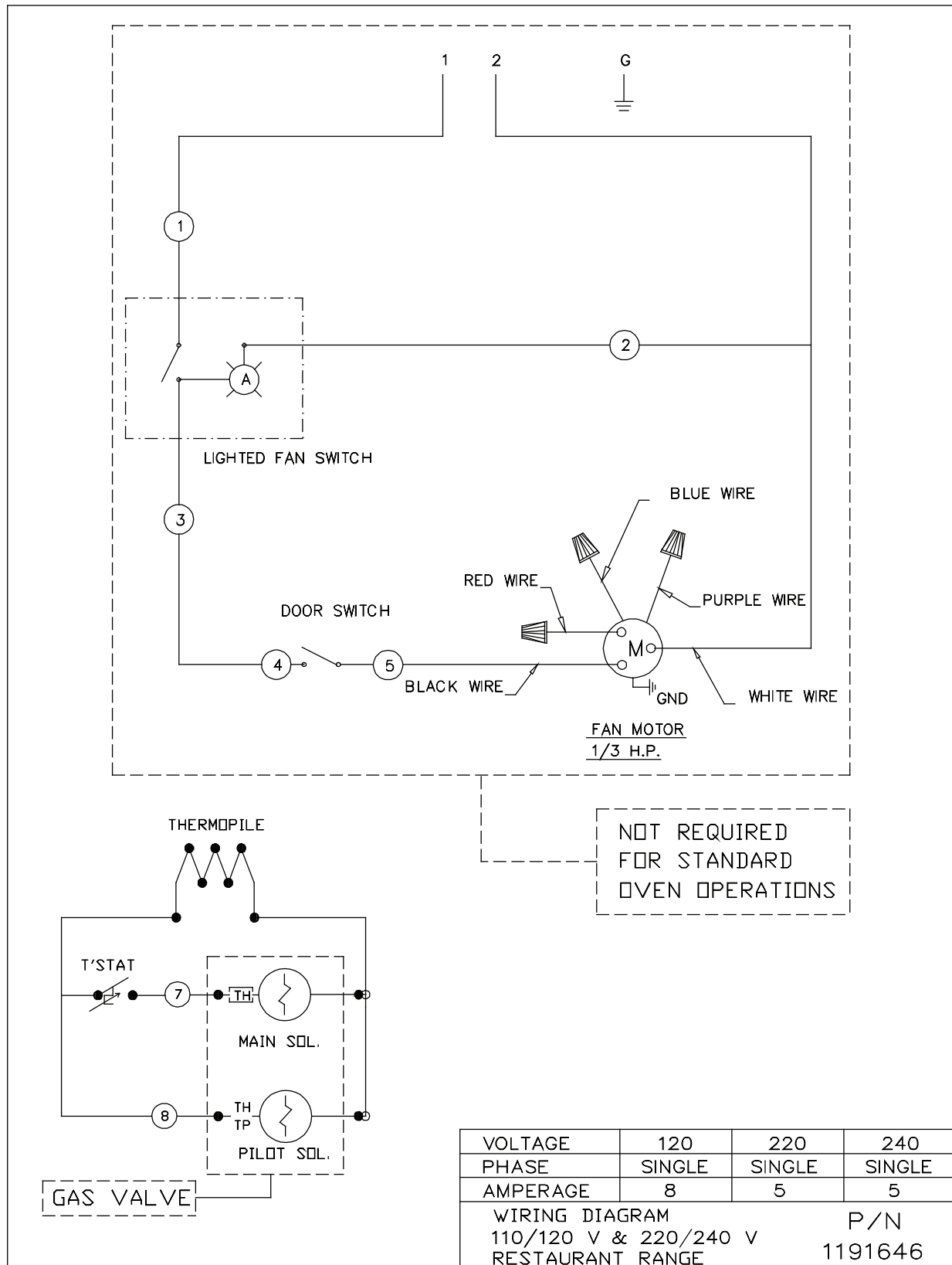
Wiring Diagram for Gas Oven
