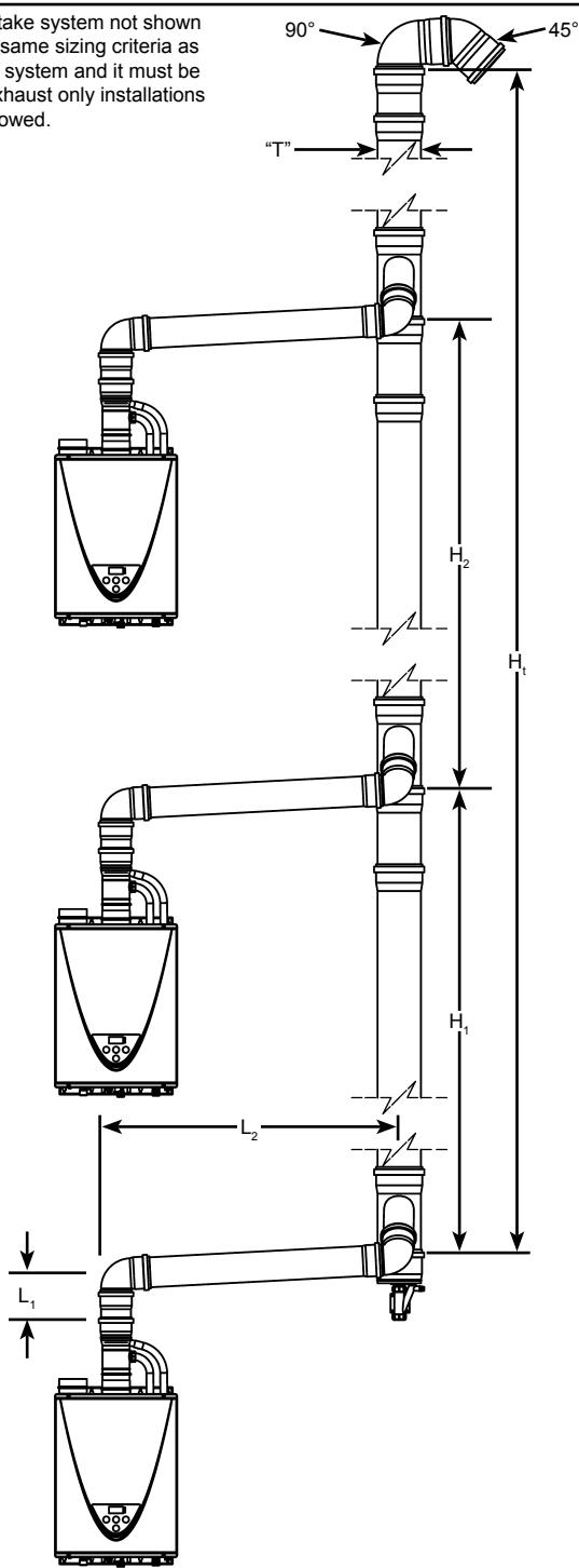
Figure 11. Vent Dimensioning
