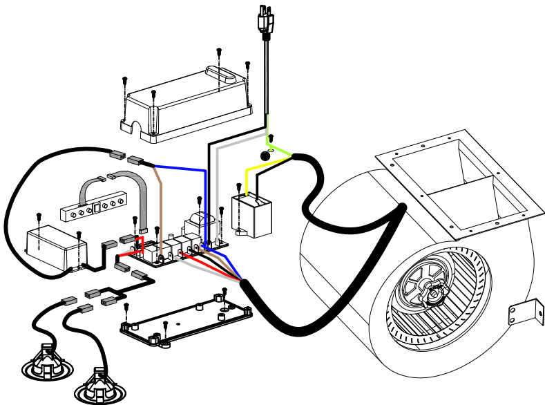
SINGLE MOTOR ELECTRICAL DIAGRAM
