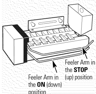
Feeler arm model
