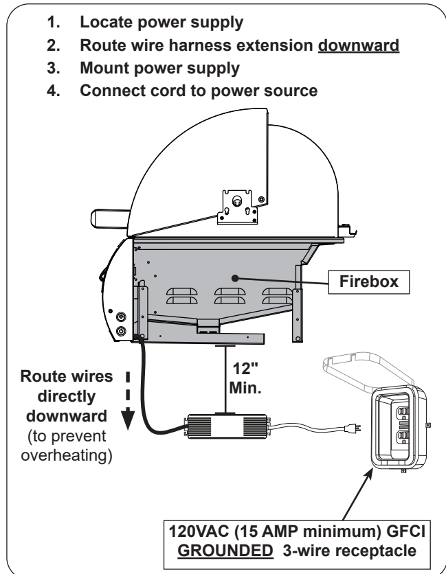
Fig. 30-3 Electrical installation
