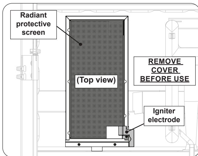
Fig. 44-1 Infrared burner overview
