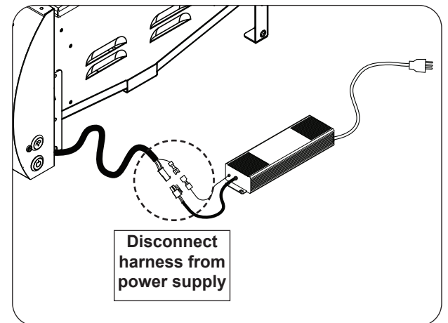
Fig. 29-2 Disconnect harness
