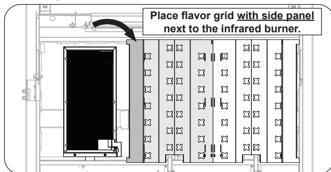
Fig. 44-4 Flavor grid placement
