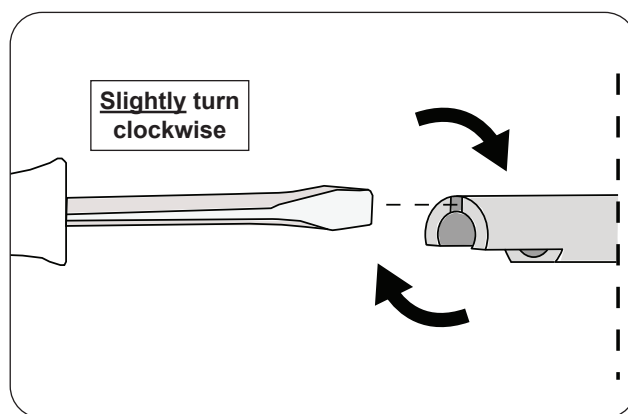
Fig. 53-2 Stem adjustment
