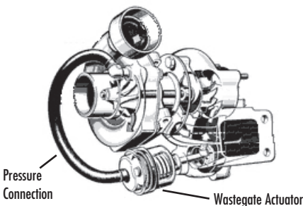
FIGURE 7: TURBOCHARGER
