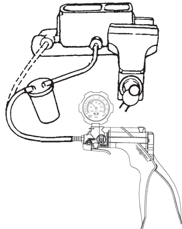
FIGURE 19: BENCH BLEEDING
