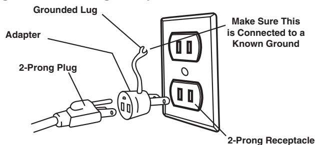
Figure 10 - 2-Prong Receptacle
