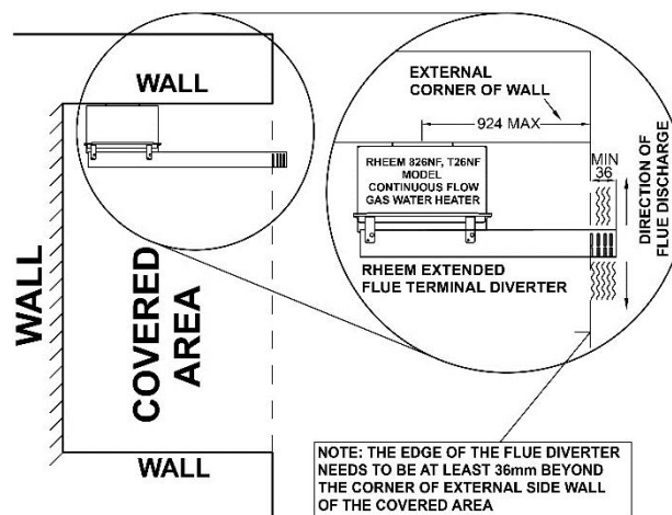
826NF or T26NF with an Extended Flue Terminal Diverter installed in compliance with AS 5601 and AS/NZS 5601.1
