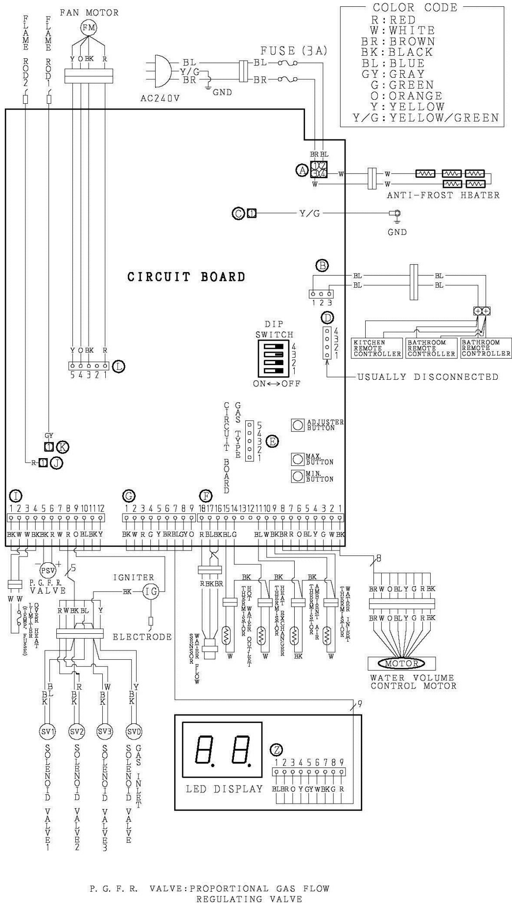
Wiring Diagram – 874, 876 Series 812, 816, T16, 820, 824, 826, T26 Models
