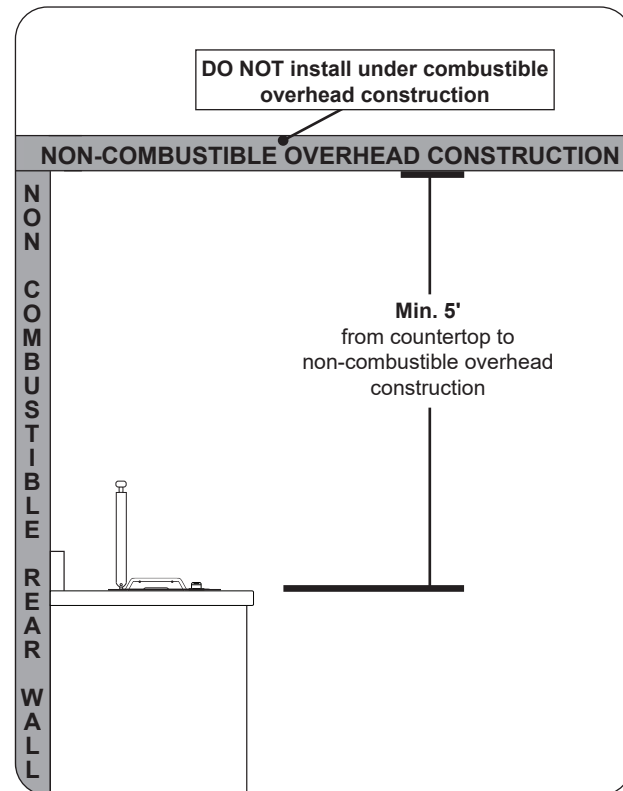
Fig. 17-1 Overhead requirements
