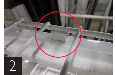
Align shelf with retainer
