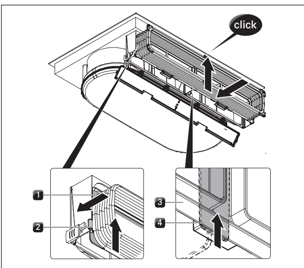
Fig. 6.15 Hooking in the frame of the flexible duct
