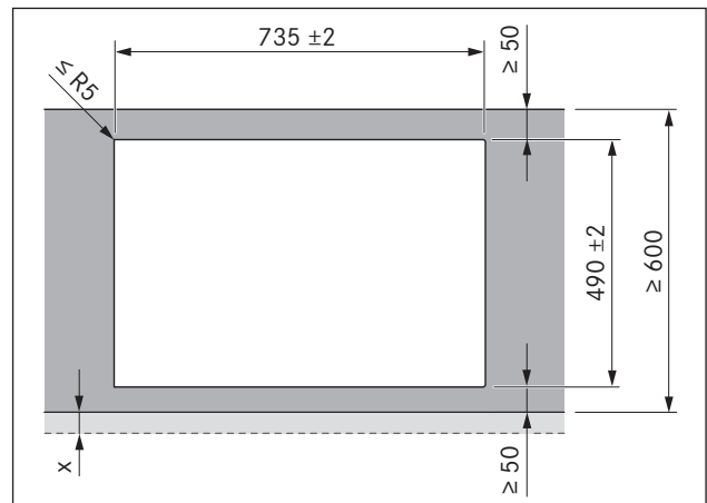
Fig. 6.5 Dimensions of cut-out for surface installation
