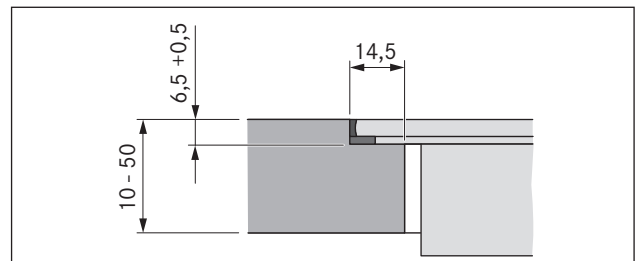
Fig. 6.4 Dimensions of groove for flush installation
