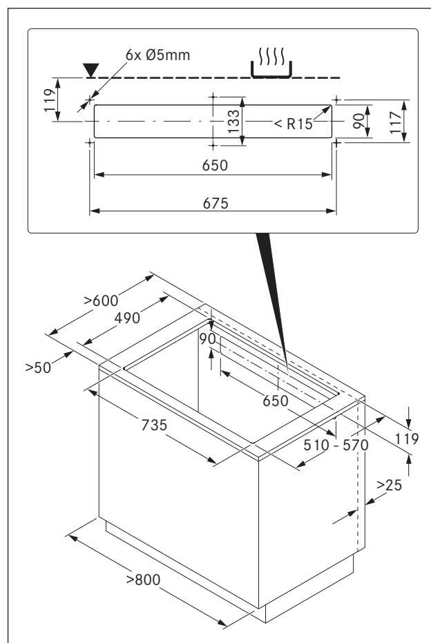
Fig. 6.9 Dimensions of furniture, recirculated air
