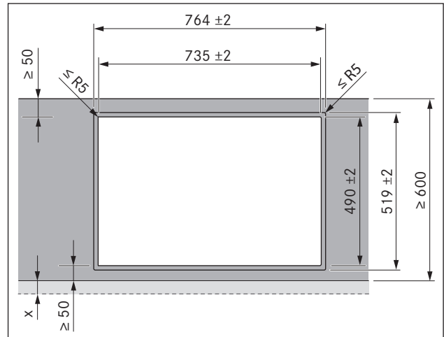
Fig. 6.3 Dimensions of cut-out for flush installation
