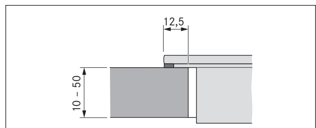
Fig. 6.6 Dimension of support for surface installation
