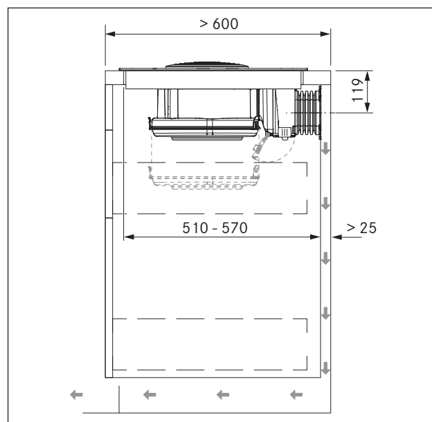
Fig. 6.10 Installation dimensions for recirculated air, worktop depth 600 mm
