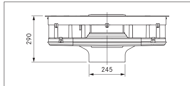
Fig. 3.2 BIA Device dimensions front view
