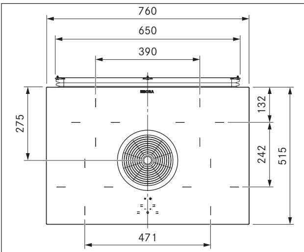
Fig. 3.5 BIU Device dimensions aerial view
