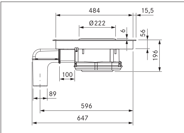
Fig. 3.4 Device dimensions with cable extension (BIA + BLAVH1)
