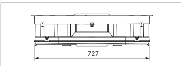
Fig. 3.6 BIU Device dimensions front view
