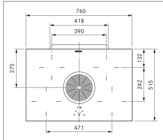
Fig. 3.1 BIA Device dimensions aerial view
