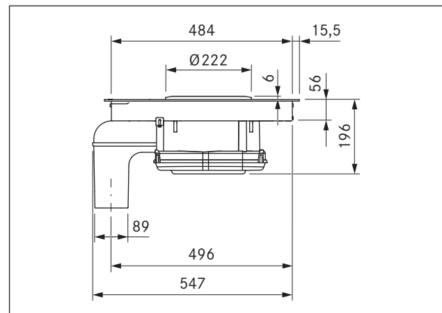
Fig. 3.3 BIA Device dimensions side view
