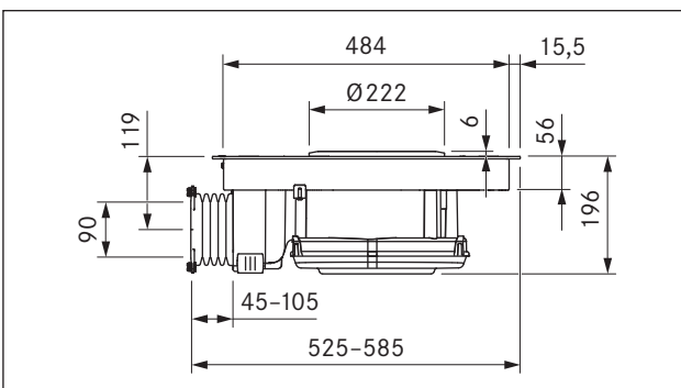
Fig. 3.7 BIU Device dimensions side view
