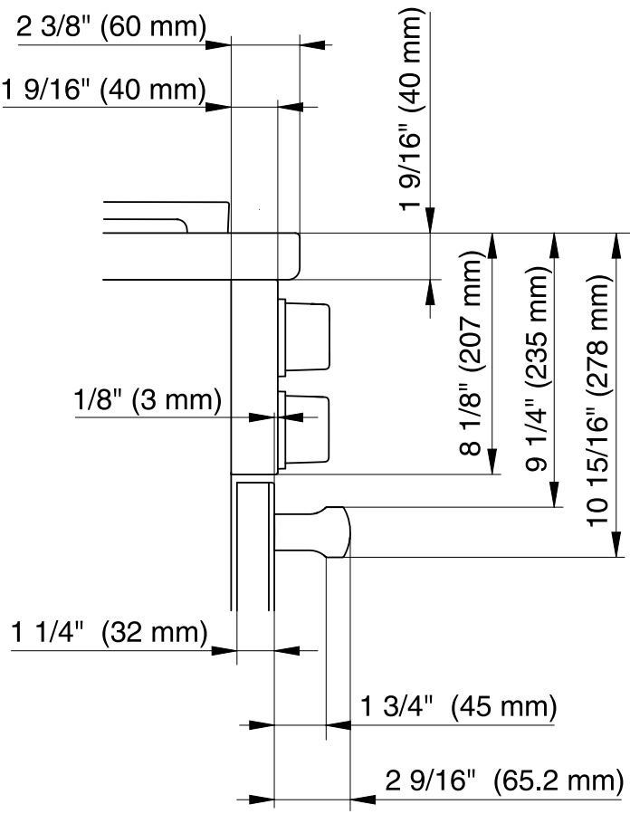
Detailed front side view of HR 1136-3 AG
