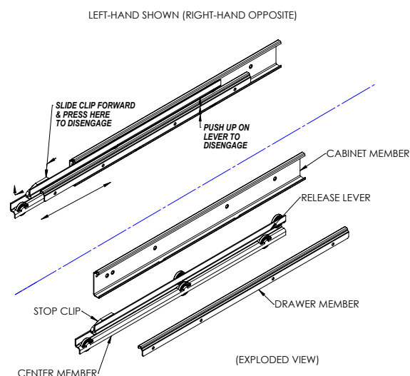
FIGURE 12: Drawer Slide
