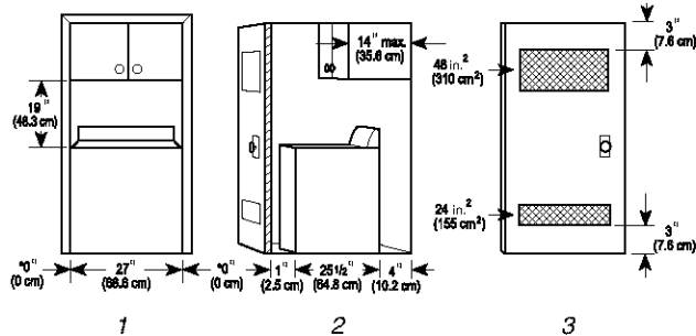
1. Front view 2. Side view 3. Closet door with vents
