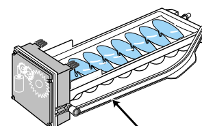
Feeler Arm
