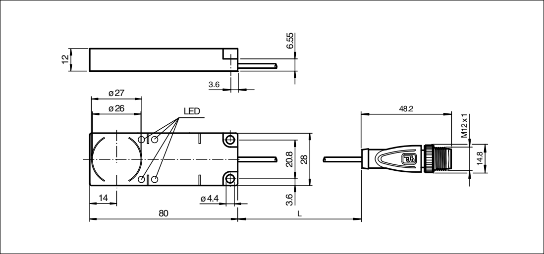
Figure 4.6 IQT4-F61-IO-V1
