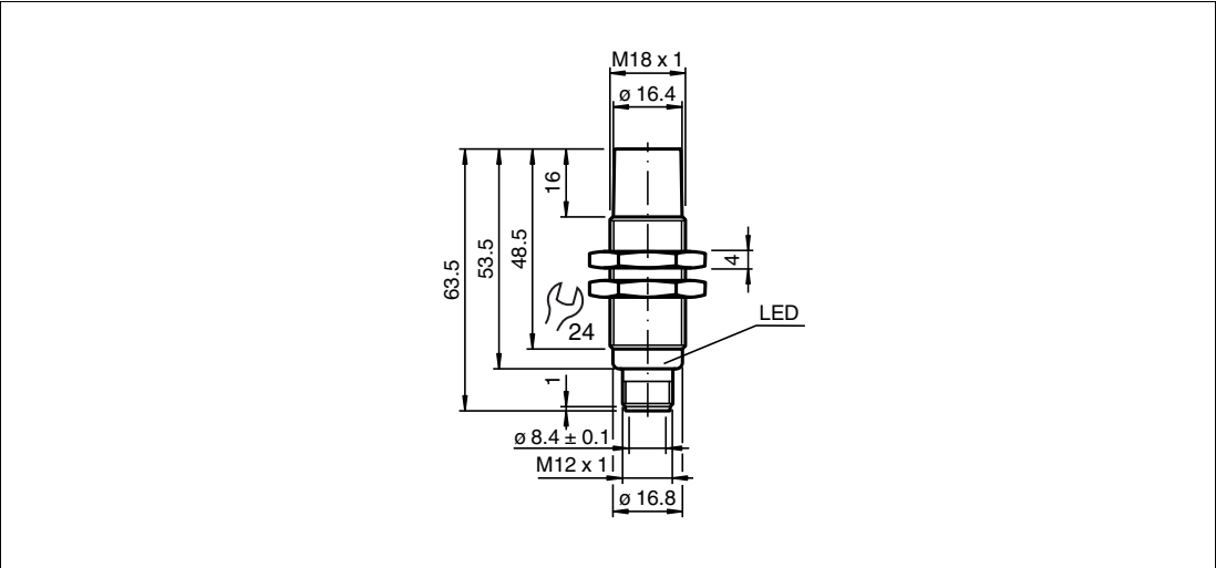
Figure 4.7 IQT4-18GM-IO-V1
