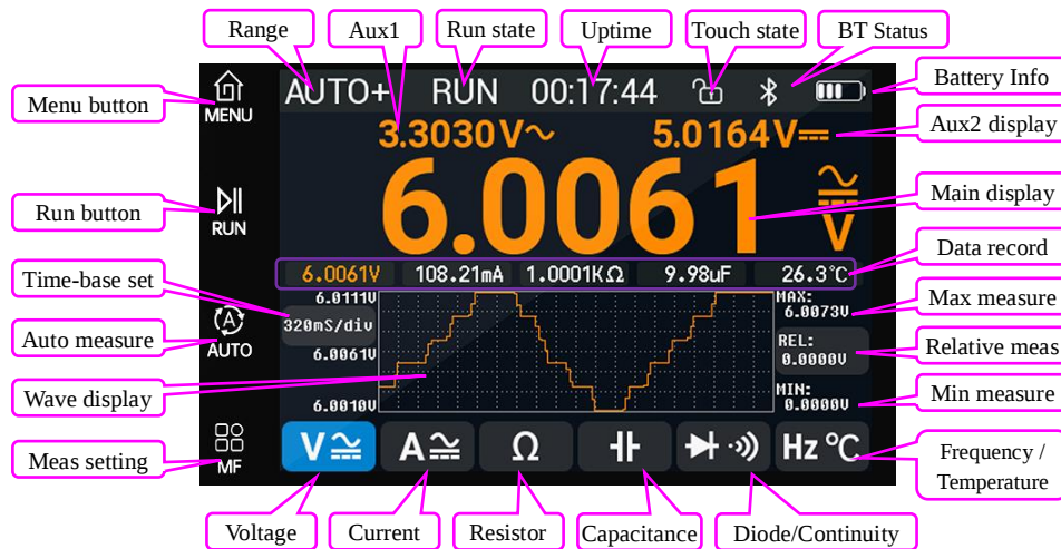
Figure 2.2.1 Multimeter measurement interface
