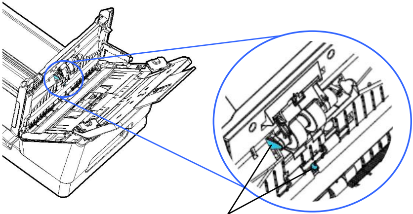
Arm Sensor
