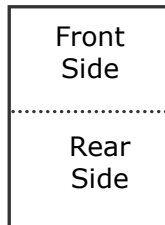
Merge Vertically
