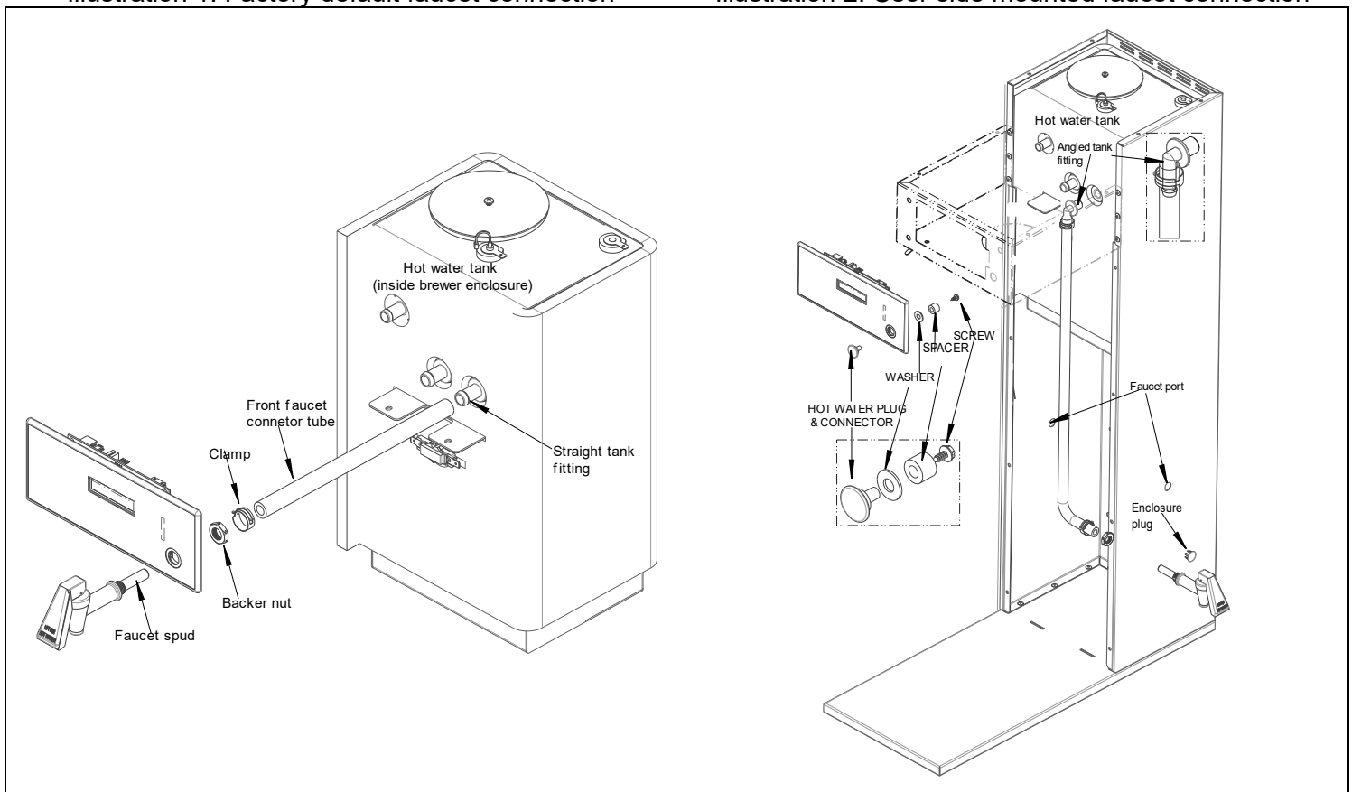
Illustration 1: Factory default faucet connection
