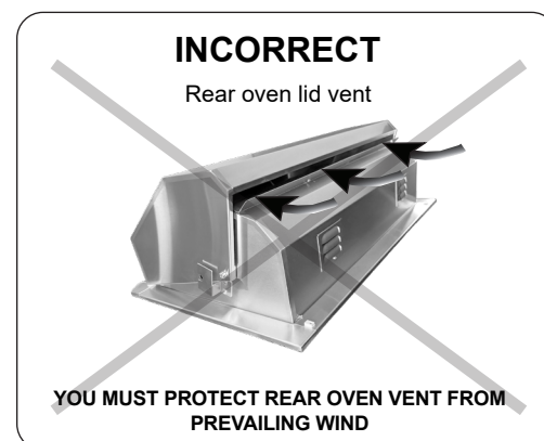
Fig. 20-4 Airflow direction - INCORRECT
