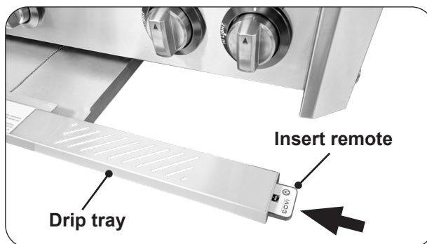
Fig. 36-2 Storage compartment
