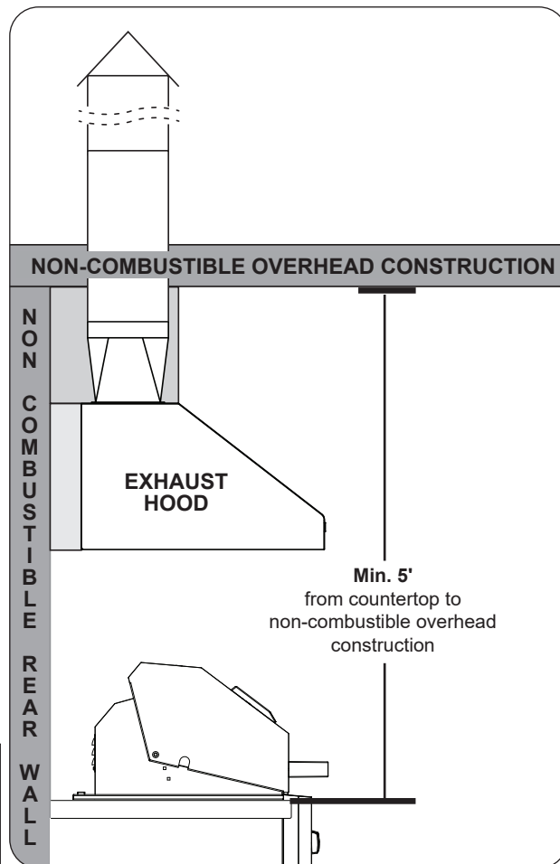
Fig. 17-1 Overhead requirements
