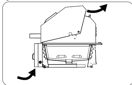
Fig. 32-1 Airflow diagram
