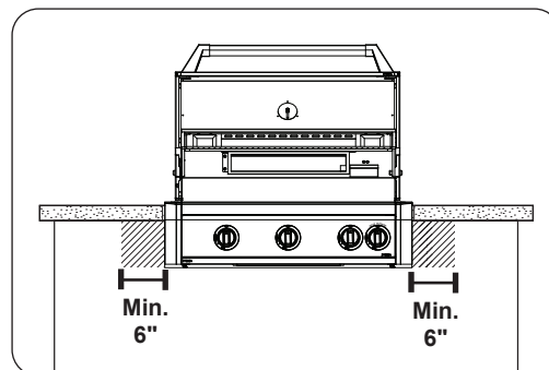
Fig. 20-1 Control panel clearances
