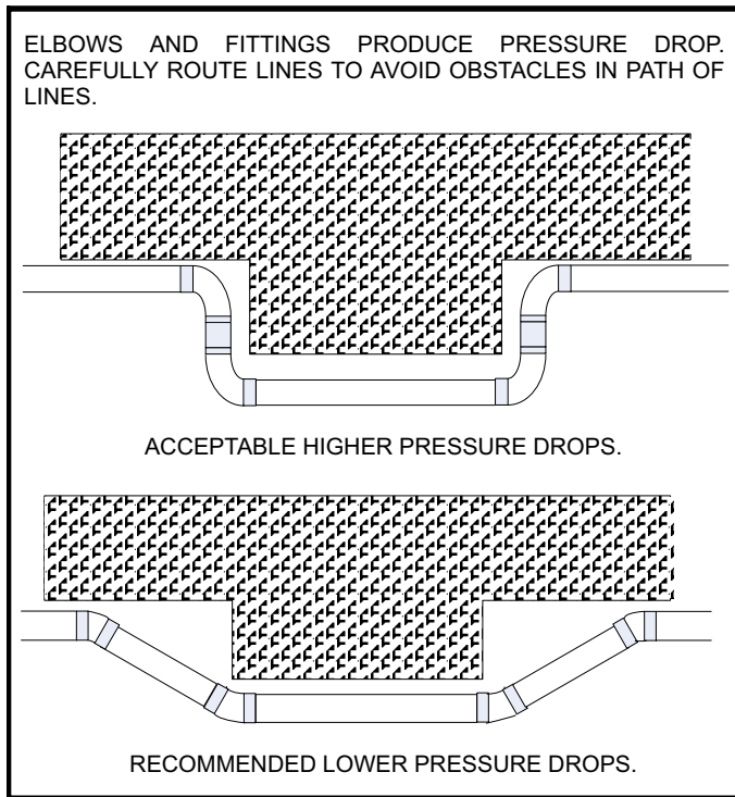
Figure 3. Pressure Drops
