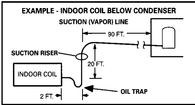
Figure 12. Indoor Coil Below Condenser
