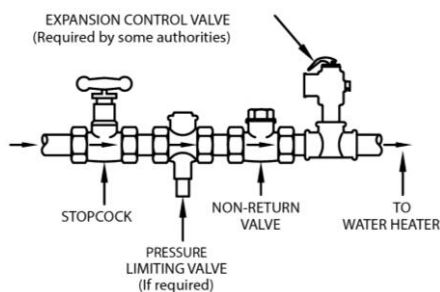
cold water connection
