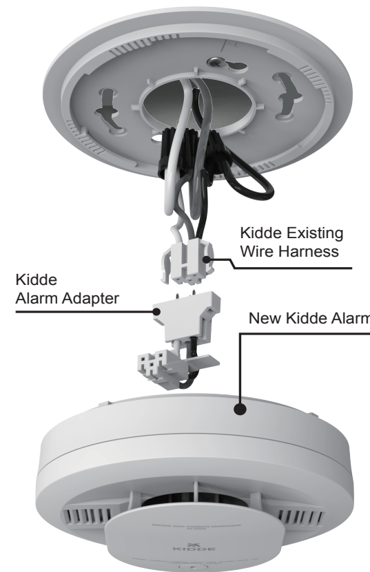
Figure 2: Adapter connecting to the old harness
