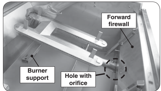
Fig. 41-3 Remove burners
