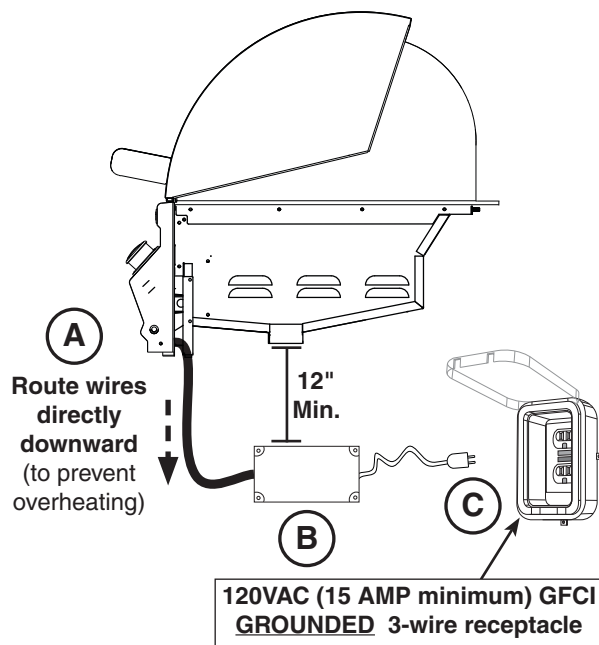
Fig. 23-1 Electrical installation
