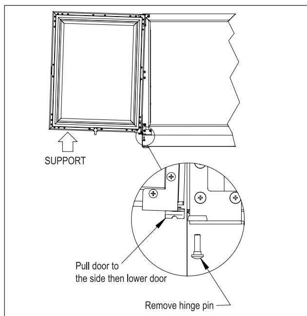
Figure 3: Door Removal
