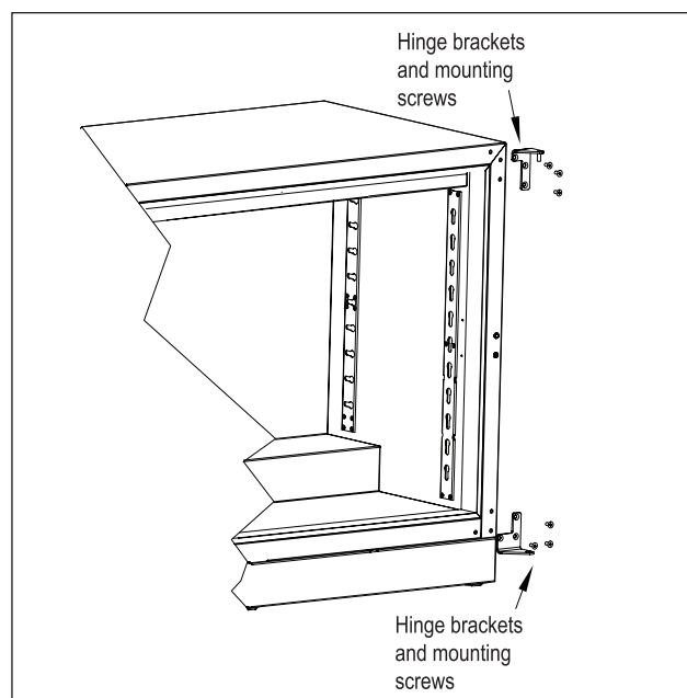
Figure 5: Hinge Installation
