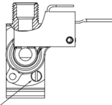
The vertical direction of the adjustment shaft groove is LP
