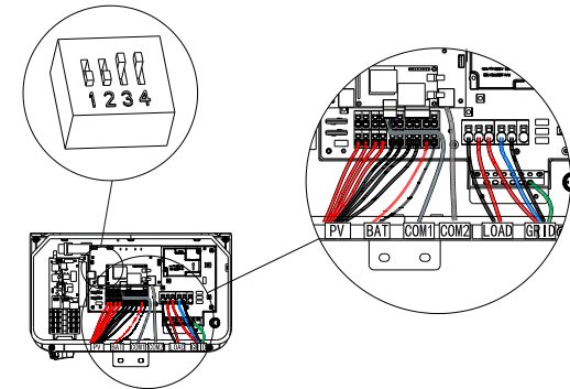
Fig 1.3 Inverter Box Wiring Diagram
