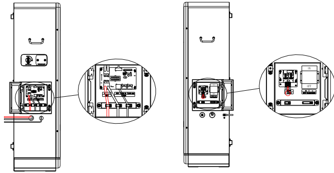
Fig 1.4 ARO Battery Wiring Diagram
