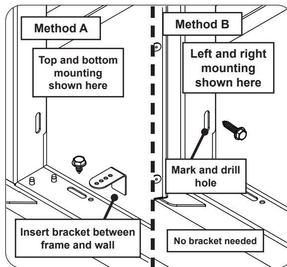
Fig. 2-3 Installation methods
