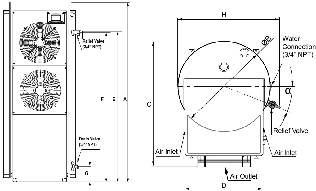
Figure 3. Rough-In Dimensions
