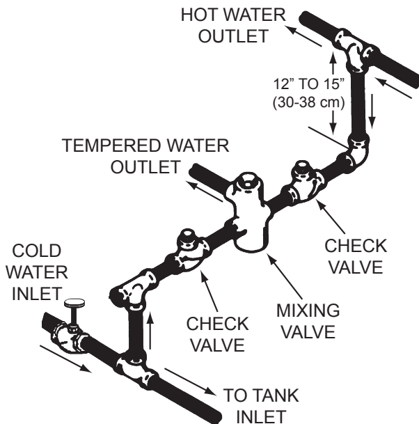
Figure 5. Mixing Valve
