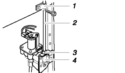
1. Tube Clamp 3. Compression Nut 2. Copper Tubing 4. Valve Inlet
