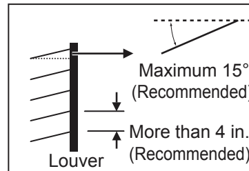
Figure 29: Louver Recommendations.
