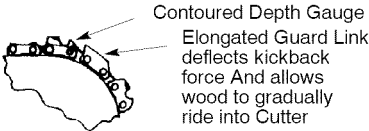
Low-Kickback Chain
