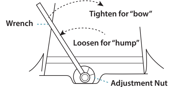
ADJUSTMENT NUT
