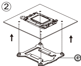
Intel Backplate
