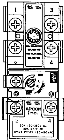
UPPER THERMOSTAT ADJUSTABLE BEHIND UPPER ACCESS PANEL
