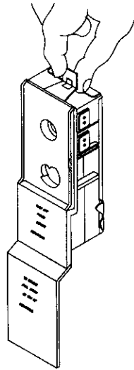
TERMINAL COVER ON UPPER THERMOSTAT
