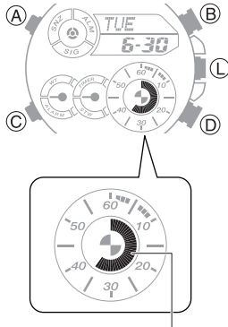
Graphic display area
