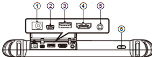
Figure 2-3 Tablet Top View
