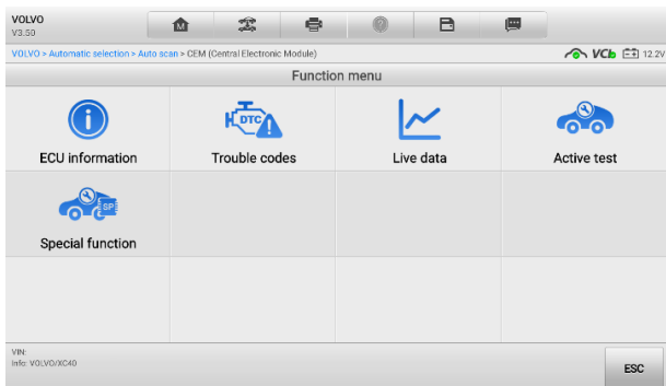
Figure 4-7 Function Menu Screen
