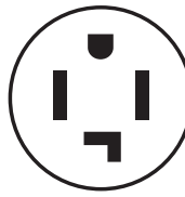
4-wire receptacle (14-30R)
