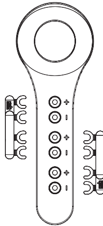
Figure 4b / Figura 4b / Abb. 4b Tri-amp / Tri-wire
