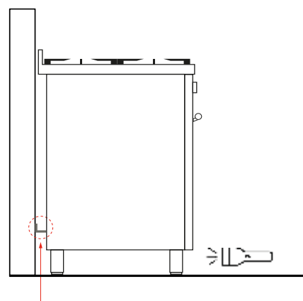
Anti-tip bracket
