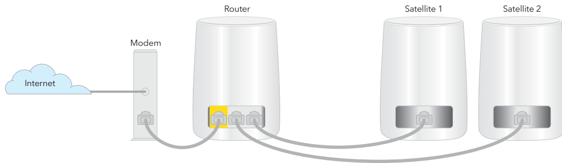
Figure 3. Star topology: Satellites connected to the router's Ethernet ports
