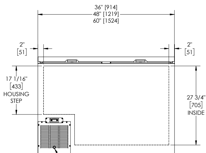
POWER CORD EXIT (BACK OF UNIT) FRONT VIEW* 36", 48", 60" CABINET
