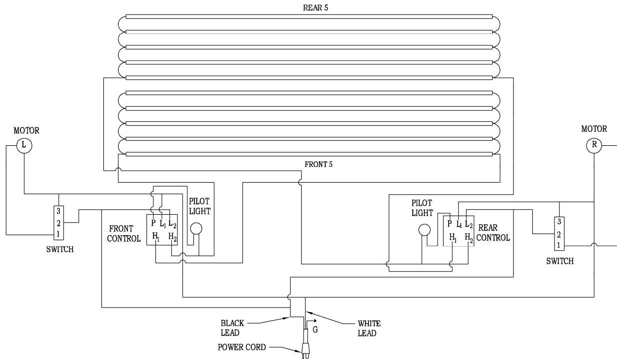
WIRING SCHEMATIC FOR ALL 8036 & 8045W MODELS
