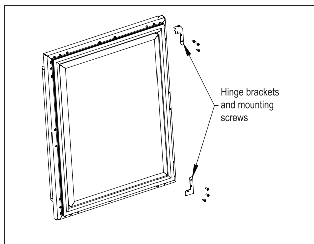
Figure 6: Door Brackets
