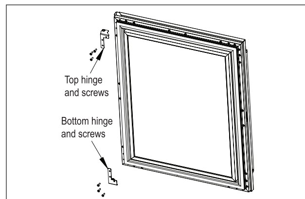
Figure 9: Door Hinges
