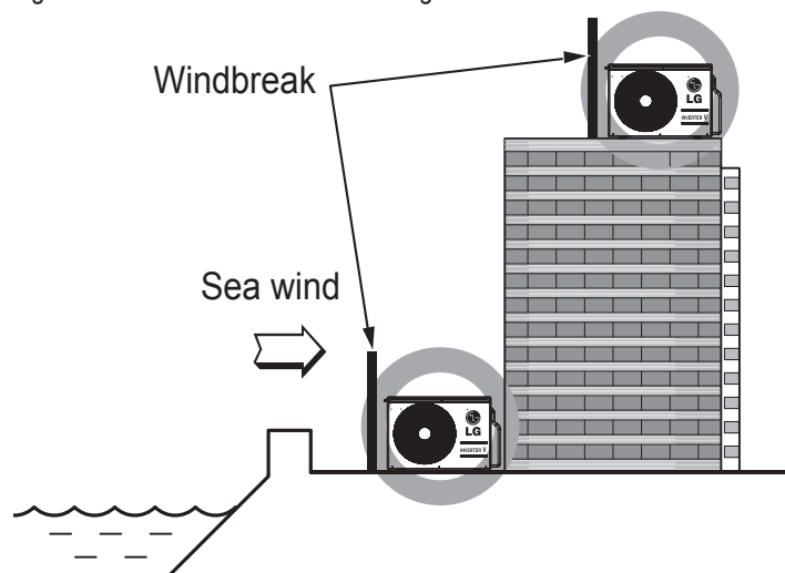
Figure 29: Oceanside Placement Using Windbreak.
