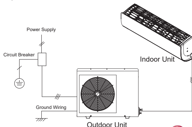
Figure 15: LS303HLV3 and LS363HLV3 General Power / Communications System Schematic.
