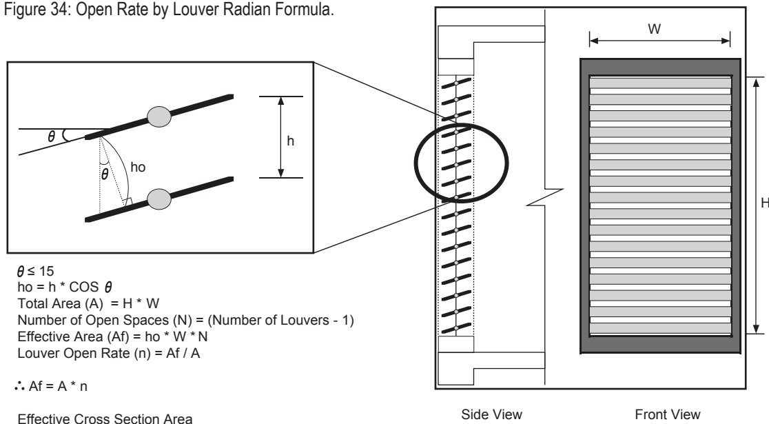
Figure 34: Open Rate by Louver Radian Formula.
