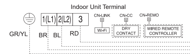
Figure 22: Wired Controller Connection (Example Only).
