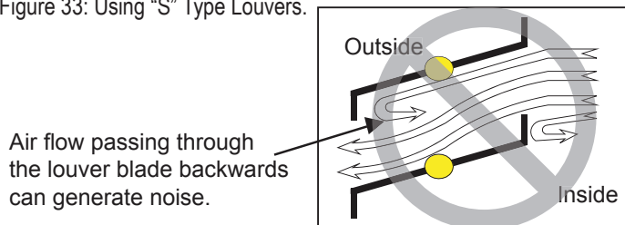
Figure 33: Using “S” Type Louvers.
