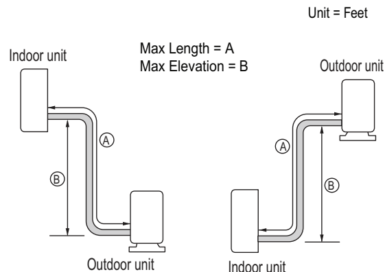
Figure 36: Single Zone Extended Piping Wall Mounted System Layout.
