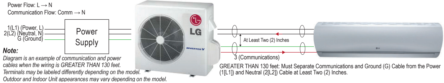
Figure 23: Schematic of a Single Zone System When the Wiring is GREATER THAN 130 Feet.
