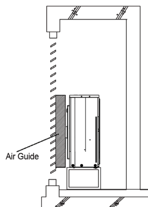
Figure 35: Example of Installing Outdoor Unit Indoors.
