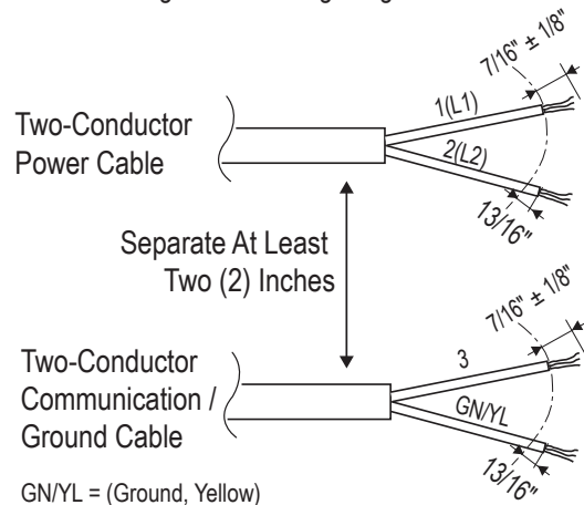
Figure 17: Single Zone Outdoor Unit to Indoor Unit Wiring and Communications Cable Diagram For Wiring Lengths GREATER THAN 130 Feet.
