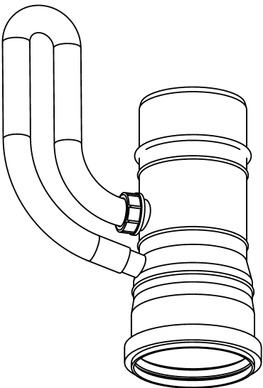
Figure 1. Clapet de non-retour (n/p 100113130)
