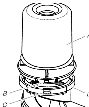
A. Dispenser assembly B. Locking tab on dispenser base C. Small slots on agitator D. Agitator assembly
